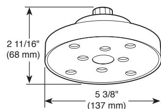
87375-▲ 1.75 GPM Shower Head
