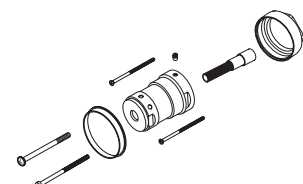
RP74785 Available Extension Kit
