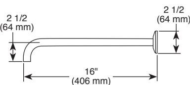
RP71648▲ Shower Arm & Flange
